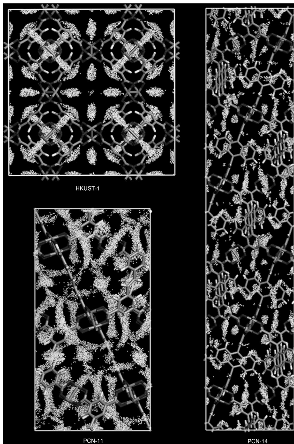
Figure 2. Probability distribution of the \text{CH}_4 center of mass in HKUST-1, PCN-11, and PCN-14 ([0 1 0] view), obtained from GCMC simulations at 298 K and 10 bar.
