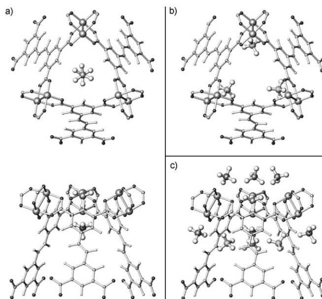
Figure 5. Experimentally determined partial structure of the PCN-11 crystal with \text{CH}_4 molecules adsorbed at a) the two cage window sites (top and side views), b) the large cage corner site I, and c) all four major adsorption sites, including the open Cu sites.
